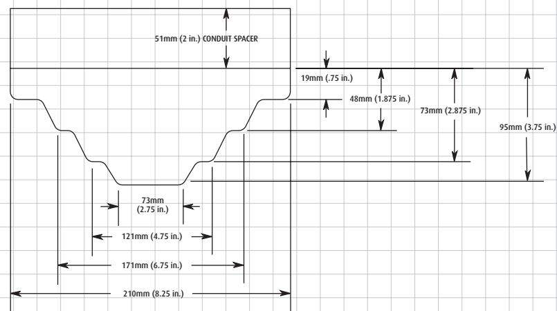
DEPTH CHART OF THE POLYCARBONATE DETECTOR STOPPER
